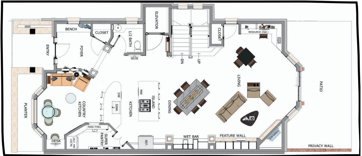
Main Floor
